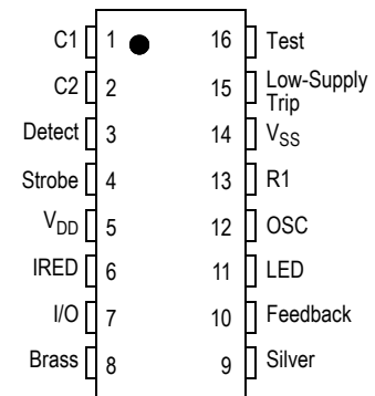
Figure 1. Pin Connections
